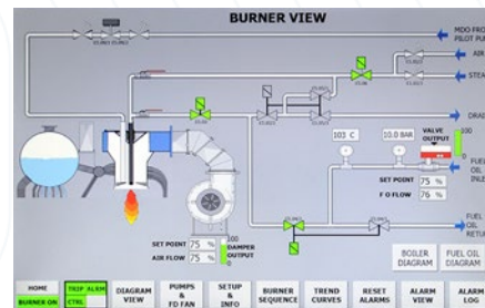
Boiler Control System
